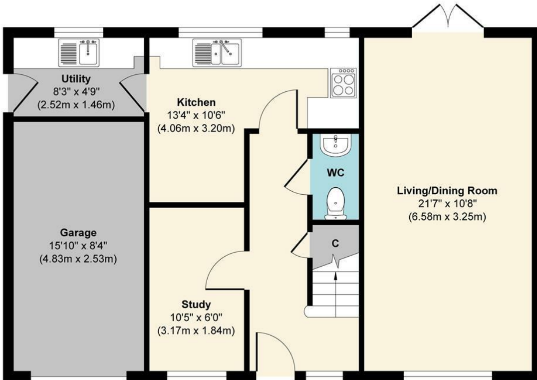
Ground Floor Approximate Floor Area 698 sq. ft (64.85 sq. m)
